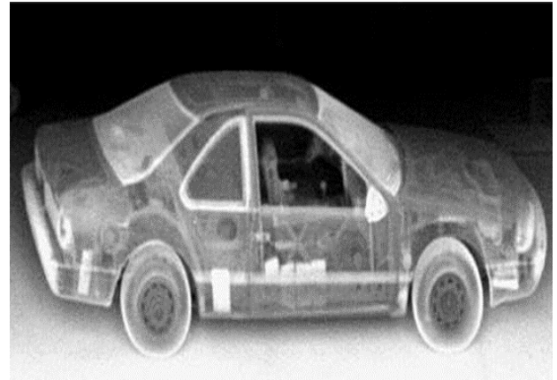
Fig 3: X-ray image of a car containing C4 explosive packages
