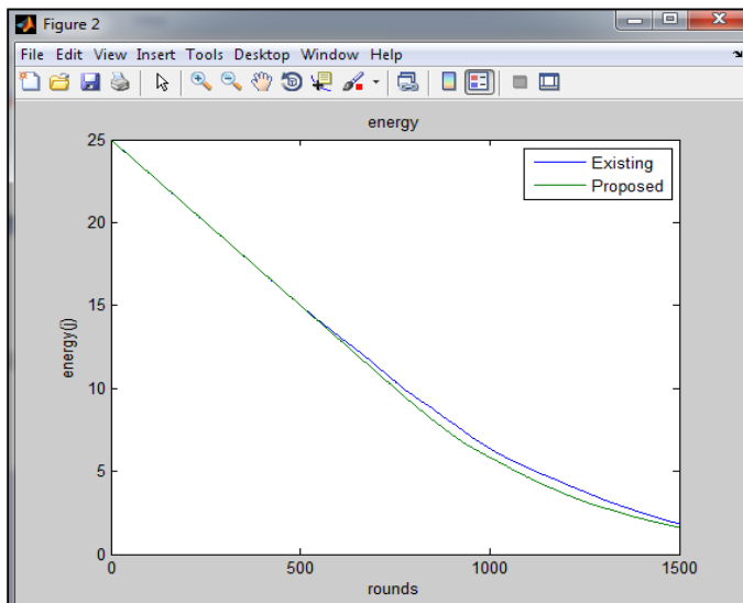
Fig 9: Comparison of the performance of existing and proposed system in terms of number of dead residual energy with total number of clustering rounds
