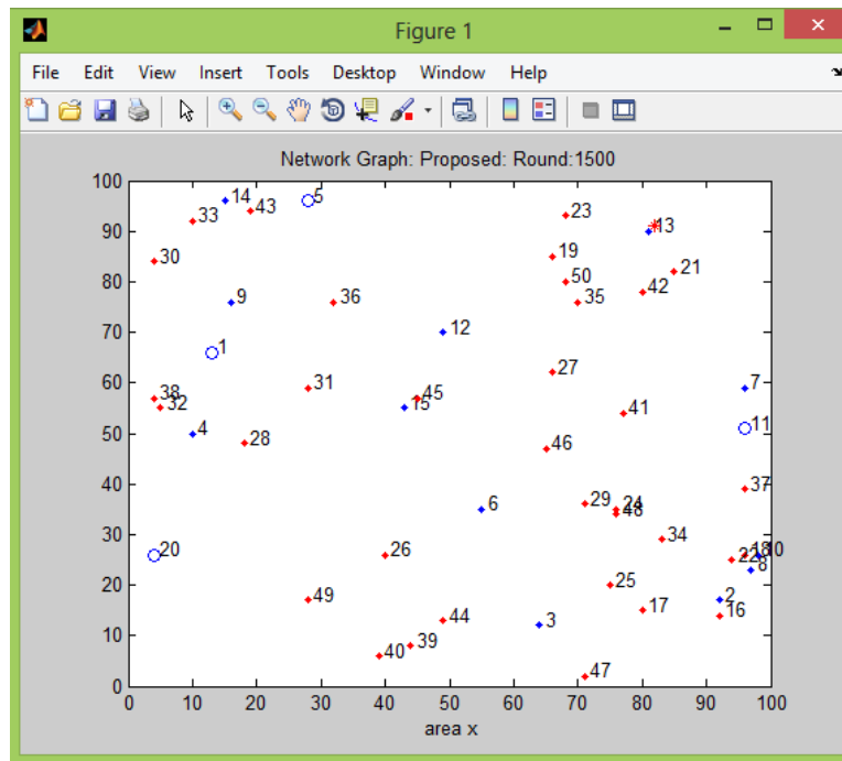
Fig 2: Cluster Formation
