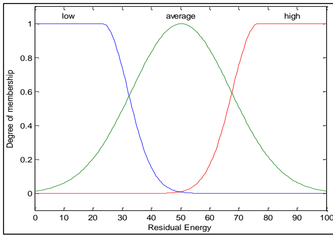
Fig 3: Degree of membership for Residual energy as first input for fuzzy system.
