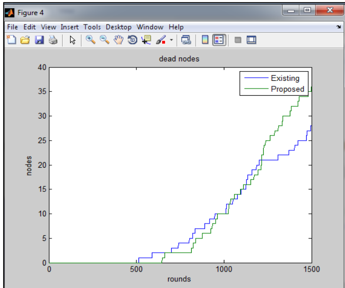
Fig 8: Performance Evaluation of existing and proposed system in terms of no. of dead nodes & no. of rounds.
