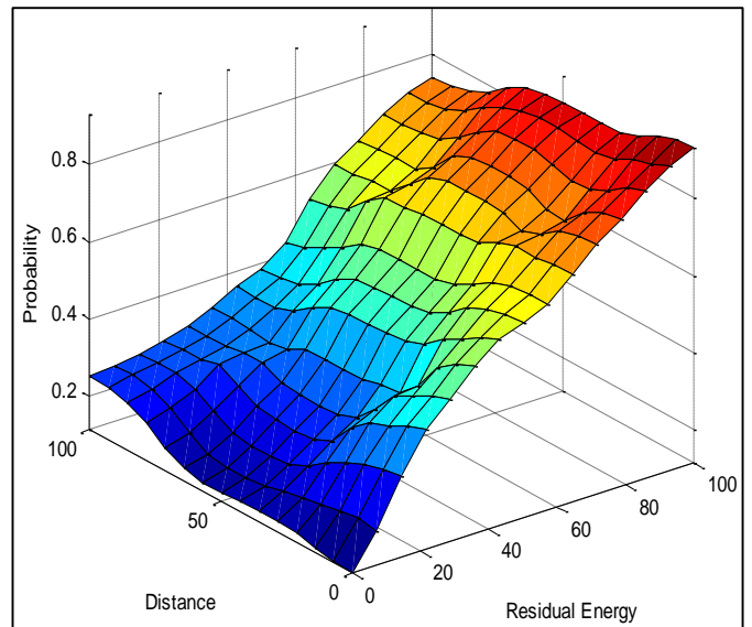
Fig 6: Surface Graph for Probability Calculation for cluster formation.
