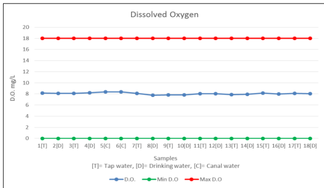
Fig 4: Dissolved Oxygen results of 18 samples taken from 6 locations in Nawabshah City
