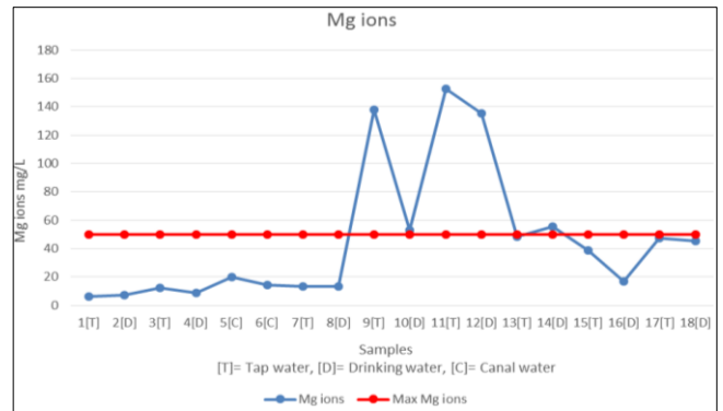
Fig 5: Magnesium Ion results of 18 samples taken from 6 locations in Nawabshah City
