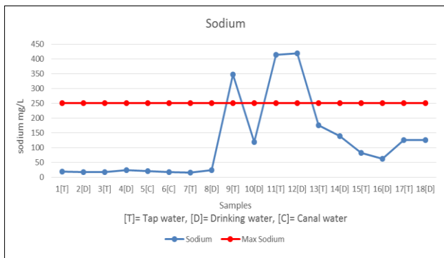
Fig 8: Sodium results of 18 samples taken from 6 locations in Nawabshah City
