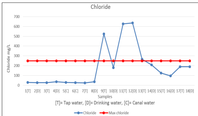
Fig 7: Chloride results of 18 samples taken from 6 locations in Nawabshah City
