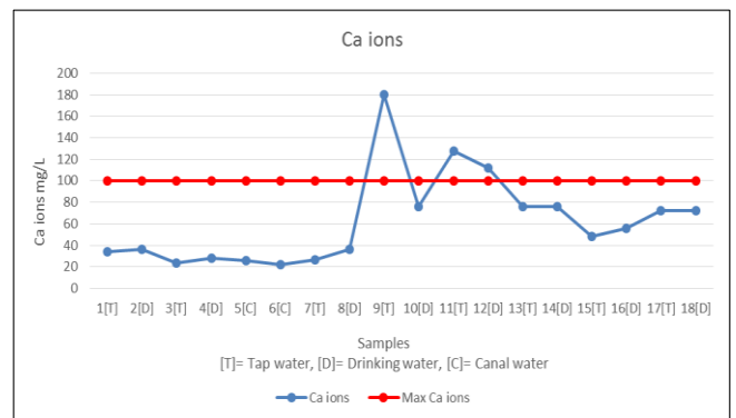
Fig 6: Calcium Ions results of 18 samples taken from 6 locations in Nawabshah City
